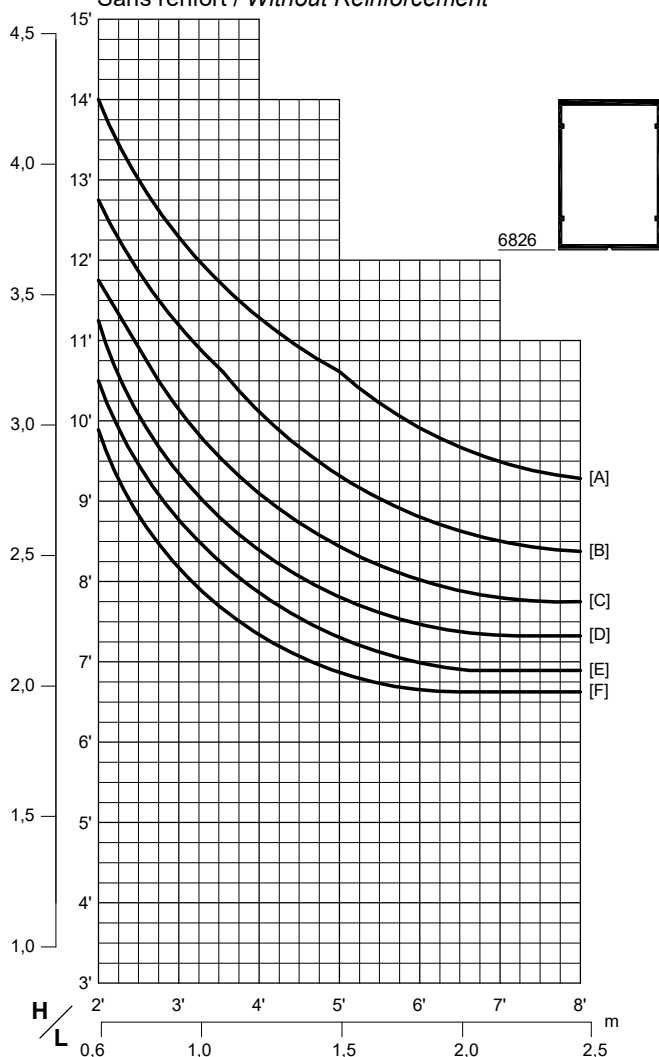
Série 6800HP Series 65mm x 100mm (2 9/16" x 4") Sans renfort / Without Reinforcement
