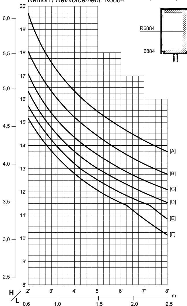
Série 6800HP Series 65mm x 100mm (2 9/16" x 4") Renfort / Reinforcement: R6884
