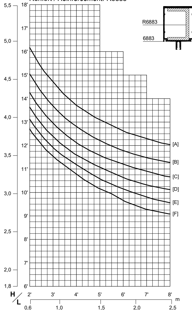
Série 6800HP Series 65mm x 75,4mm (2 9/16" x 3") Renfort / Reinforcement: R6883
