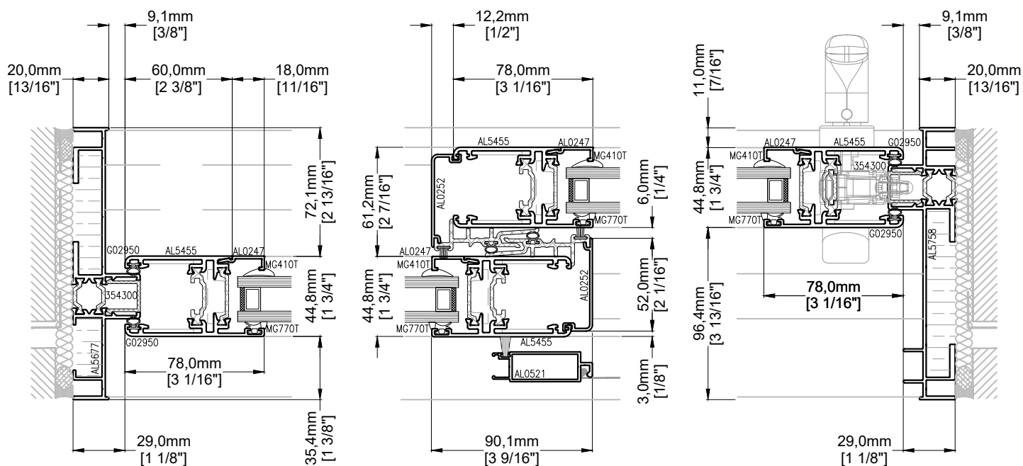
Panneau fixe Fixed panel
